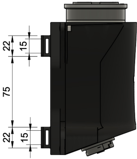
Pole Mounting
