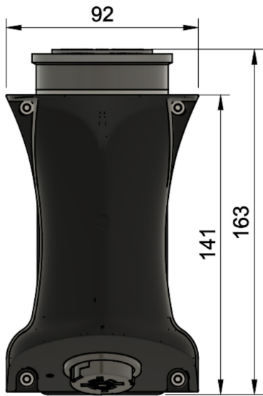
Pole Mounting
