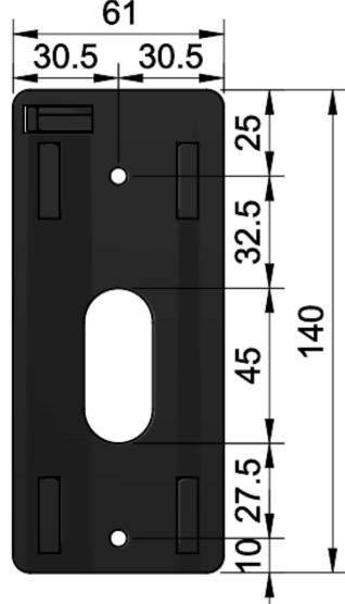
Wall Mounting
